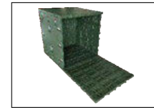
ITEM : RPG3590 Material:PE ID: L820xW820xH820mm OD: L900xW900xH900mm
