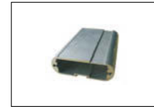
ITEM:AEH151 Material:AL SIZE:W72.5×H24×L100 mm
