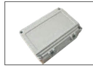
ITEM:AW046 Material:AL SIZE:L220×W155×H96 mm
